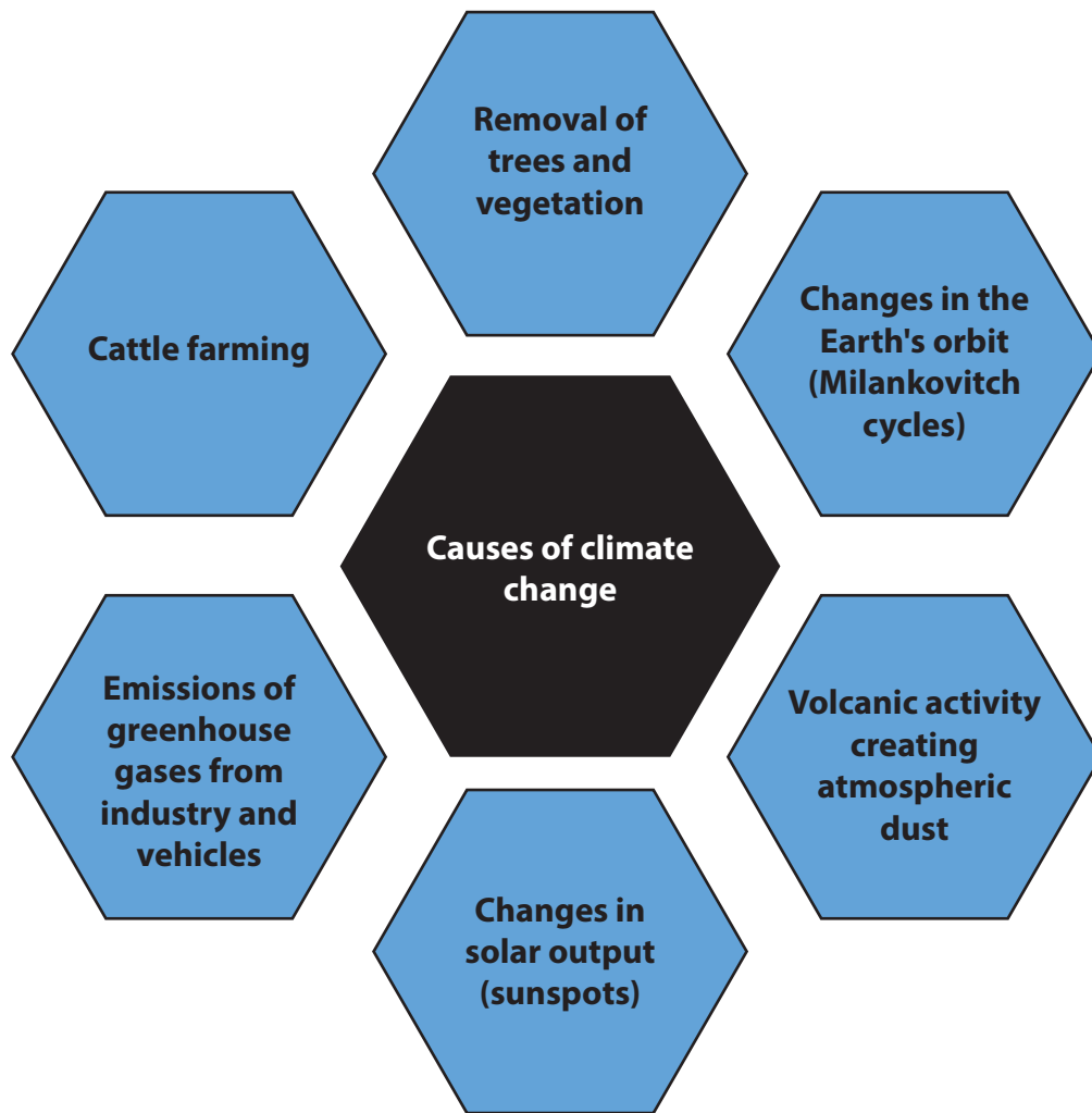
Figure 7c Selected causes of climate change
