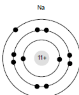
Sodium atom with electronic configuration of 2.8.1
